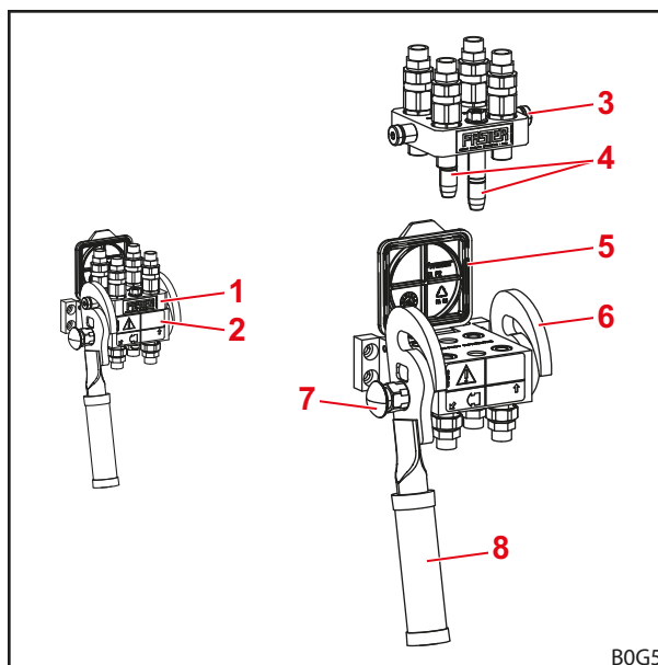
Obr. 22 Spojka Hydro-Fix
