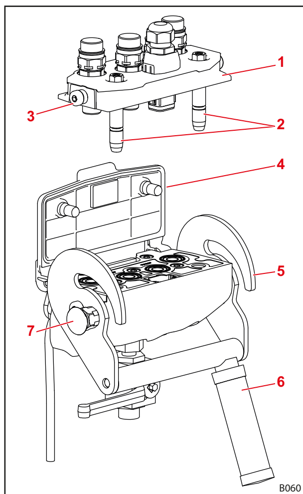
Fig. 77 Hydro-Fix
