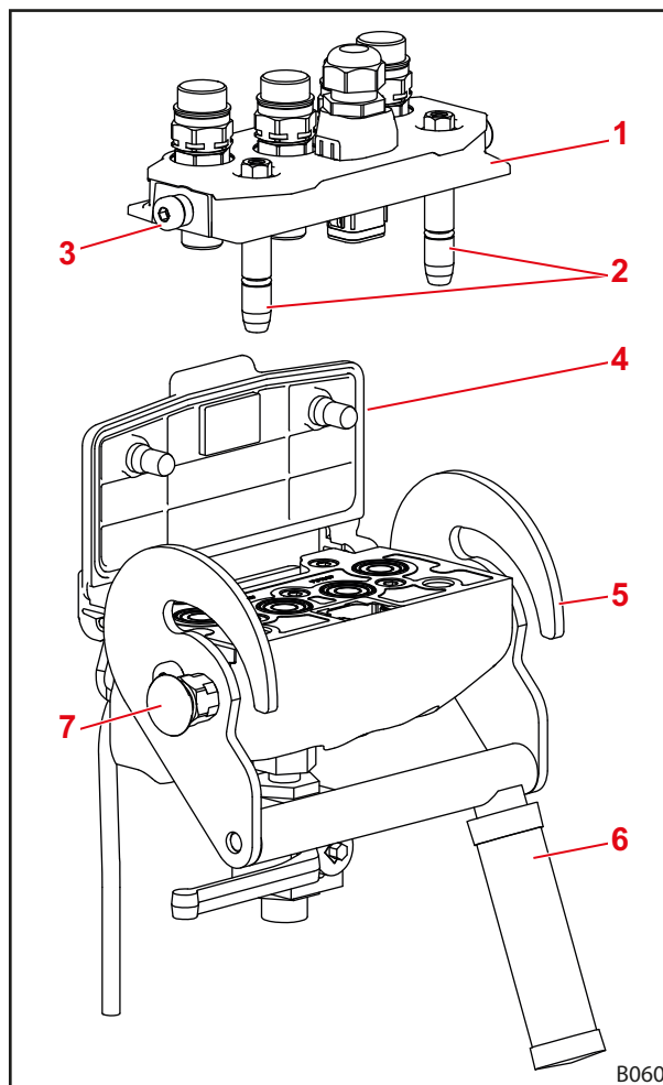
Obr. 81 Hydro-Fix
