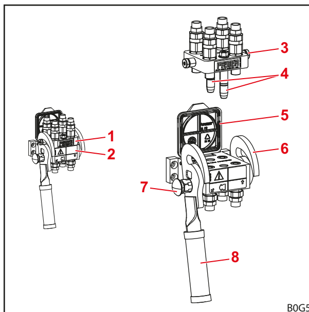
Obr. 22 Hydro-Fix
