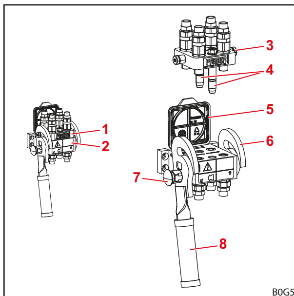
Fig. 22 Hydro-Fix
