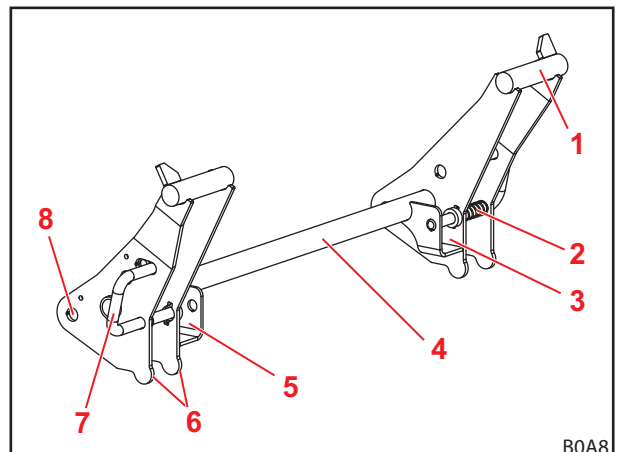
Fig. 17 Euro-wisselframe
