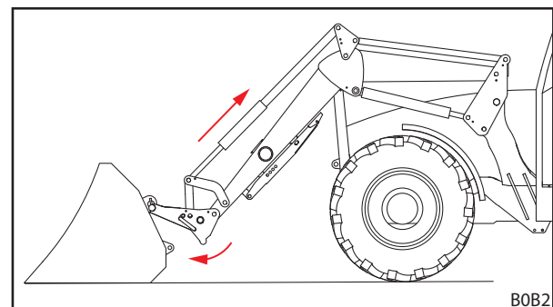
Fig. 91 Inhaken
