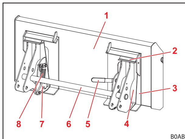
Fig. 25 Geopende vergrendeling
