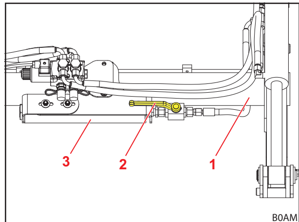
Fig. 47 Mechanisch bediende Comfort-Drive (hendelpositie Comfort-Drive-aan)
