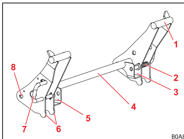
Fig. 27 Euro-wisselframe
