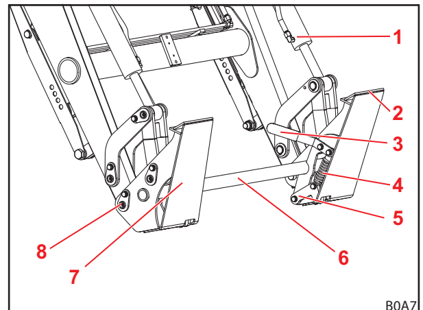
Fig. 16 Skid-Steer-wisselframe
