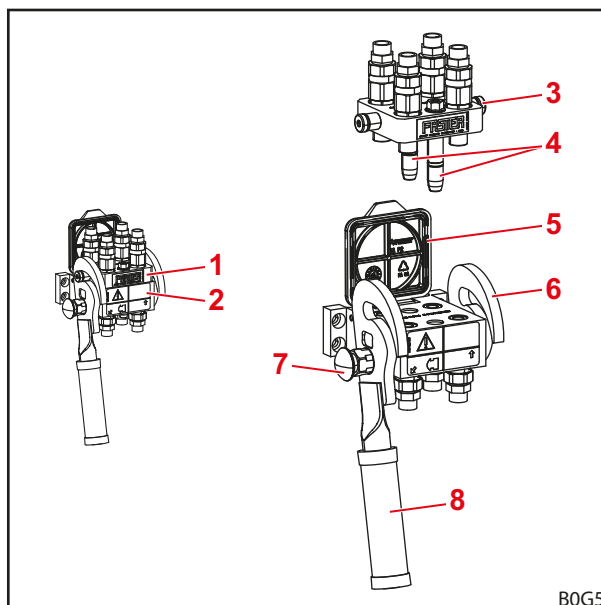
jn 22 Hydro-Fix
