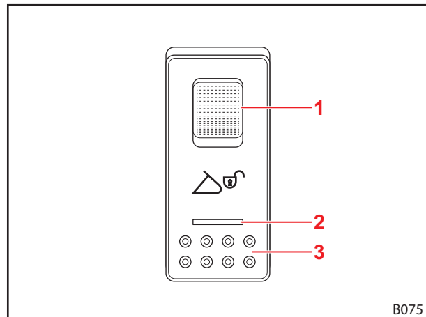
Abb. 91 Hydro-Lock-Schalter
