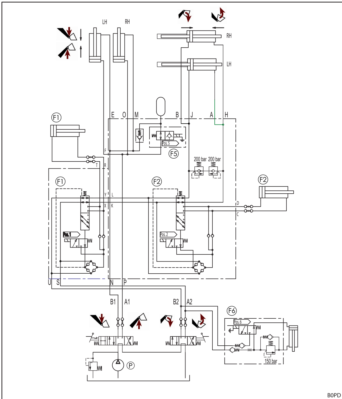
Abb. 132 Hydraulikplan TL
