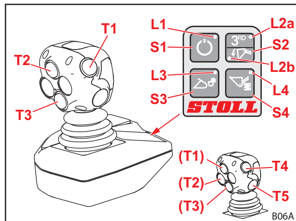
Abb. 72 STOLL Pro Control
