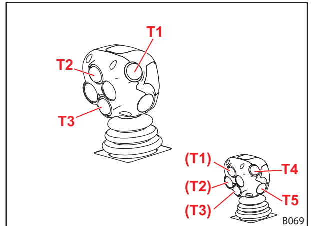
Abb. 74 STOLL Trac Control (3 Taster)
