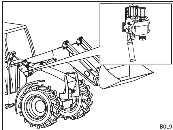
Abb. 19 Hydro-Fix: Position am Frontlader
