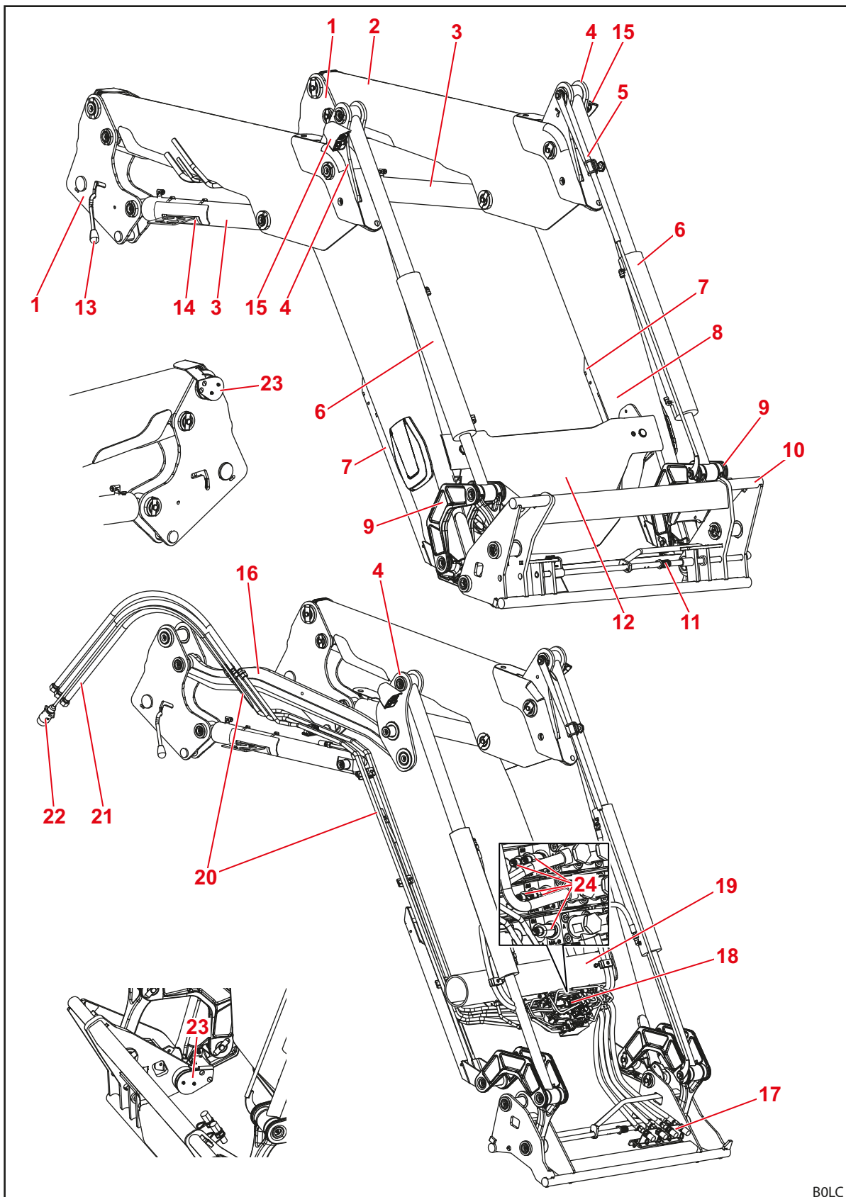
Abb. 8 Frontlader FZ IB+
