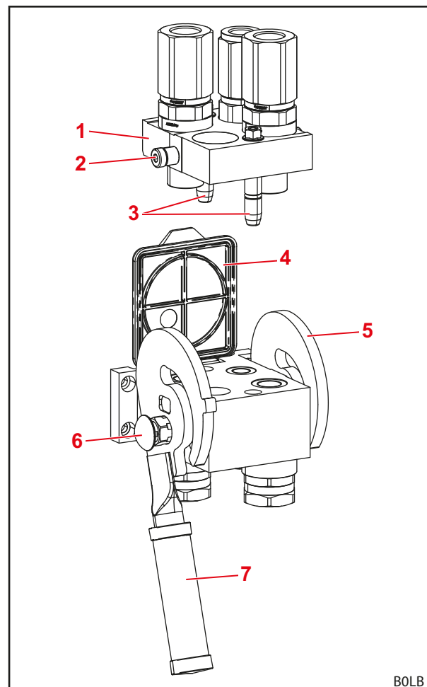
Abb. 74 Hydro-Fix
