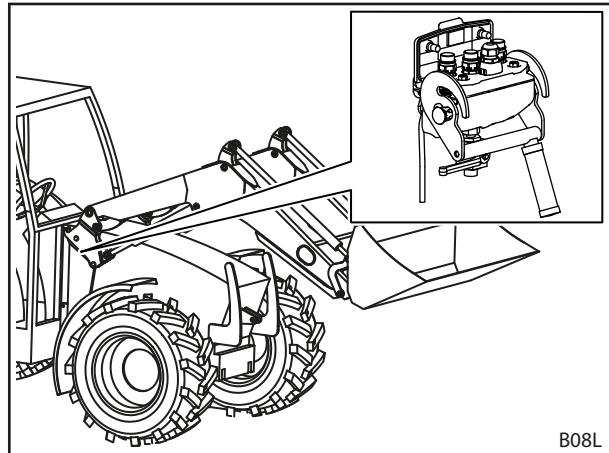
Abb. 22 Hydro-Fix: Position am Frontlader
