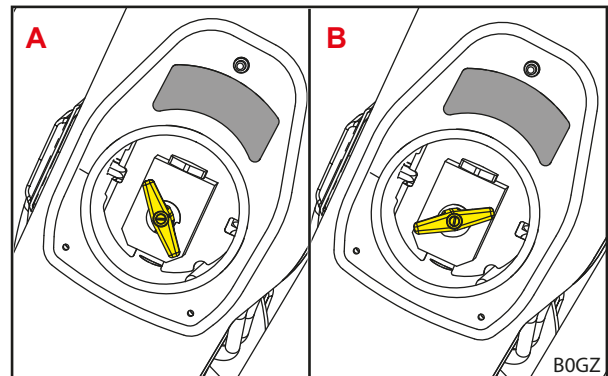
Abb. 42 Hebelstellungen Comfort-Drive
