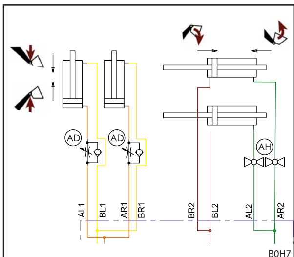
Abb. 148 Hydraulikplan Absenkdrössel
